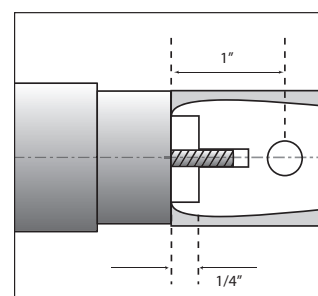
Bottle Stopper Chuck
