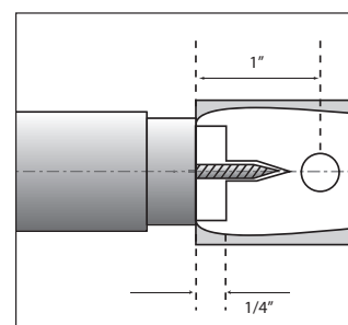
Small Screw Chuck
